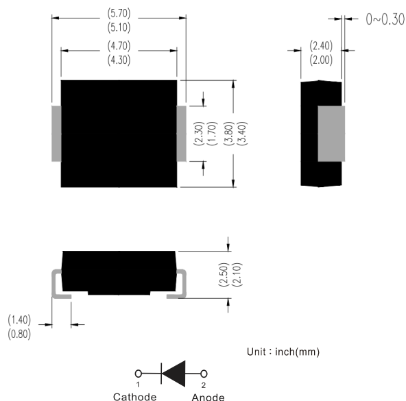
SMB/DO-214AA
